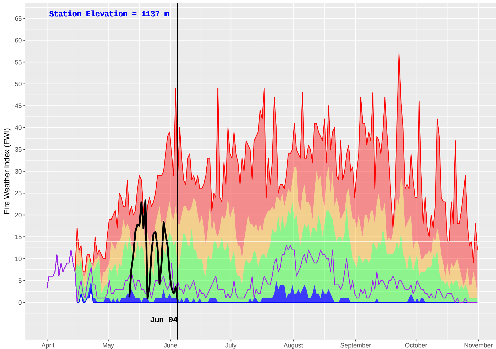
KLUSKUS (166) : Historical (1982–2016) and Current (2018) Noon Fire Weather Index (FWI)
