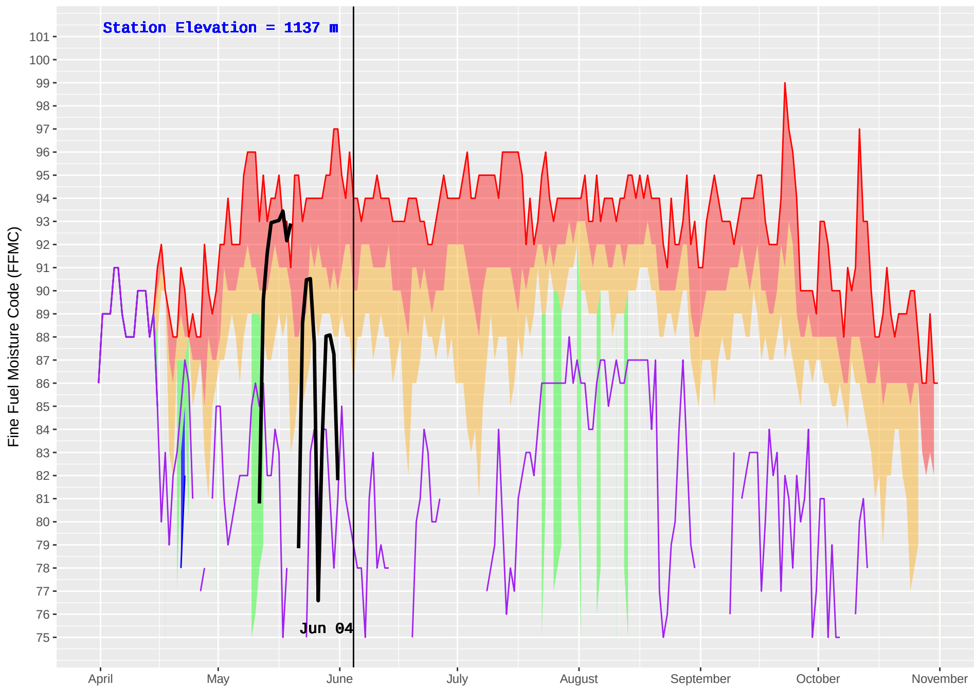
KLUSKUS (166) : Historical (1982–2016) and Current (2018) Noon Fine Fuel Moisture Code (FFMC)
